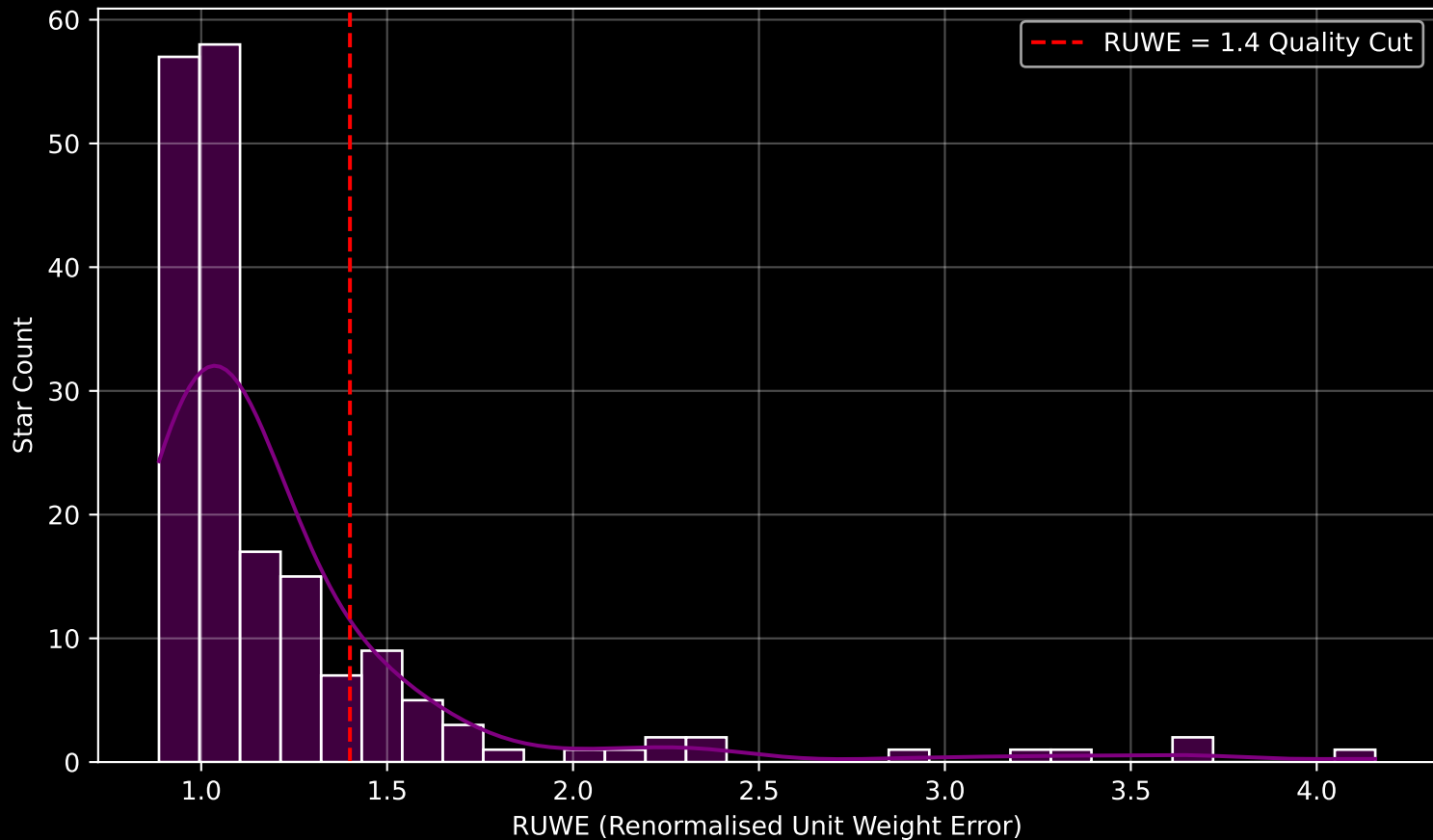
GAPOGEE DR17 Field [K2_C8_140-55] RUWE Distribution (n= 184)
