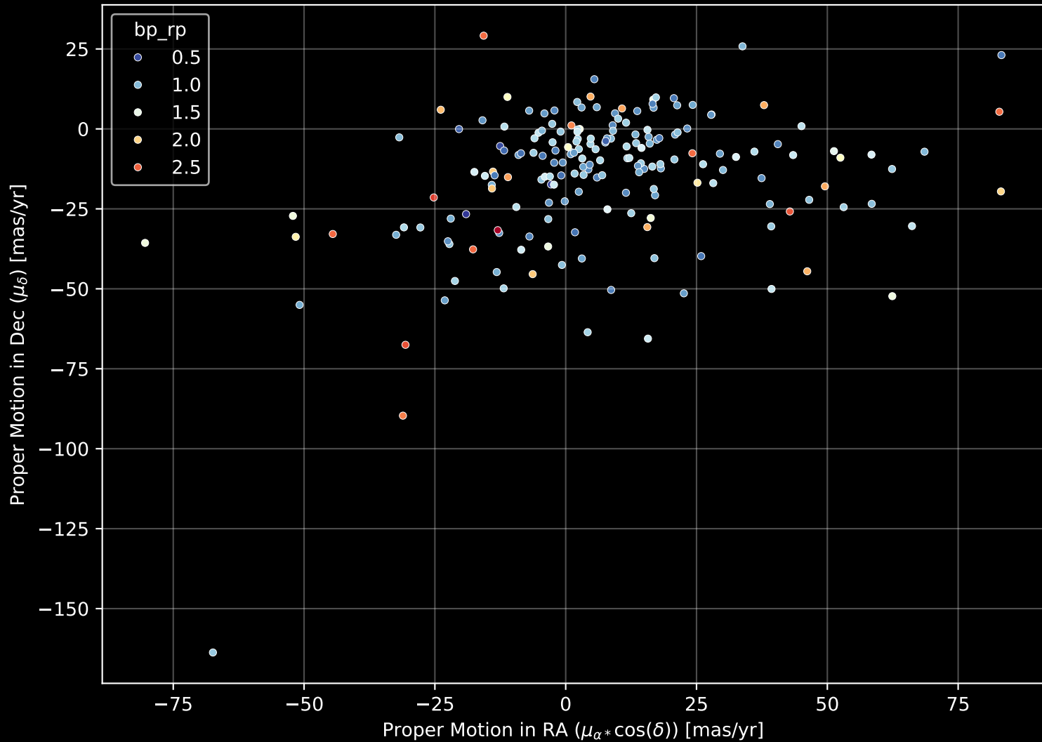
APOGEE DR17 Field: [K2_C8_140-55] Proper Motion Diagram (n= 189)
