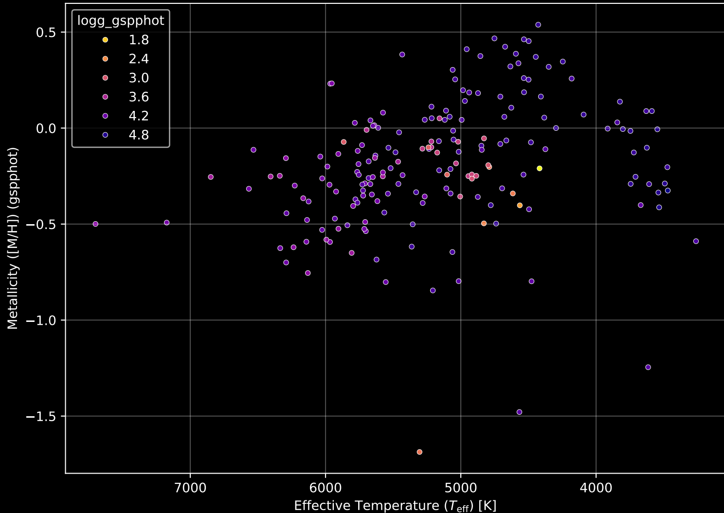
APOGEE DR17 Field: [K2_C8_140-55] Stellar Population Parameters (n= 189)
