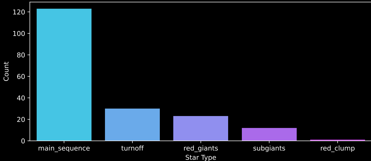
APOGEE DR17 Field: [K2_C8_140-55] Count plot of Star Type
