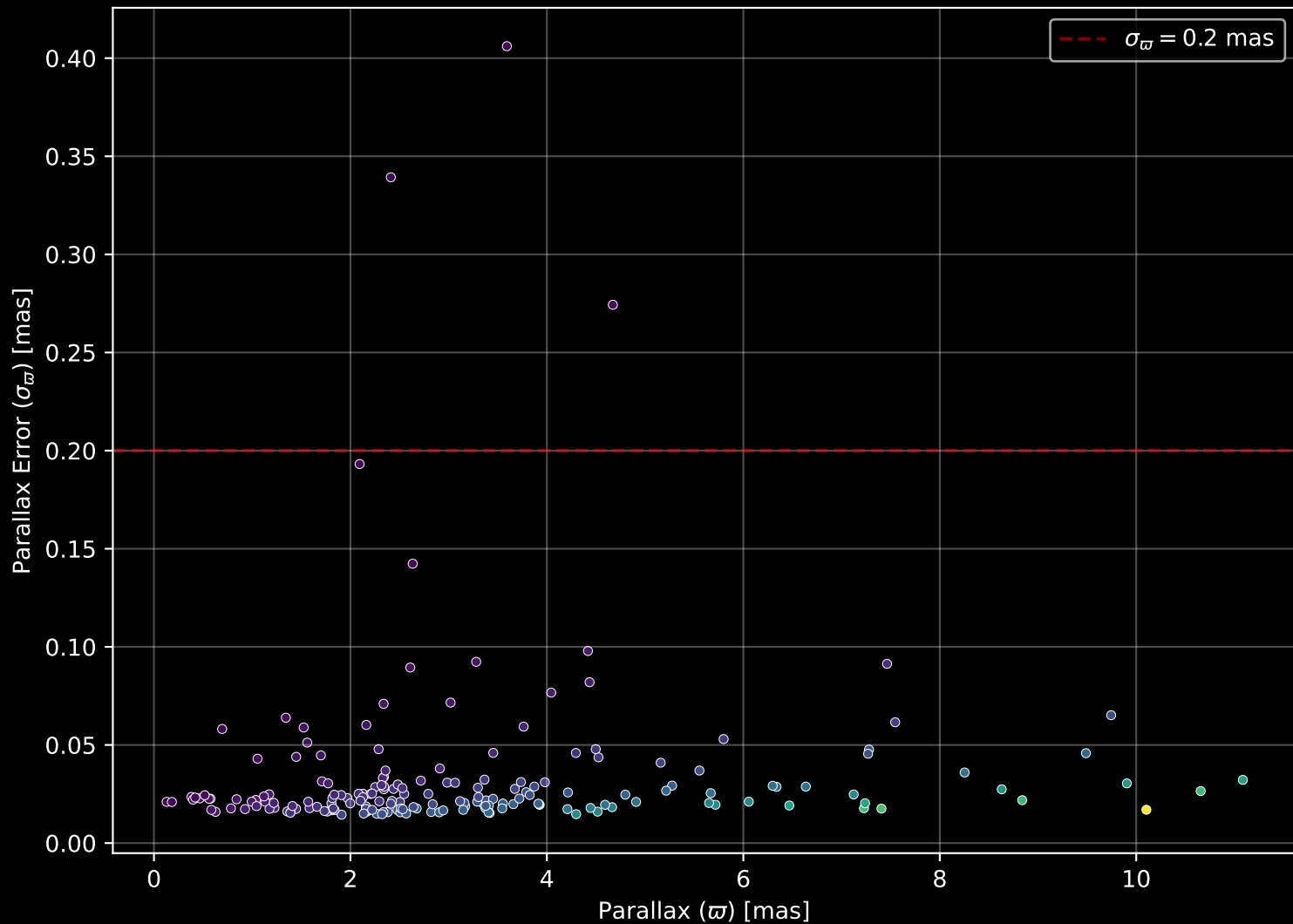
APOGEE DR17 Field: [K2_C8_140-55] Parallax Quality (n= 189)
