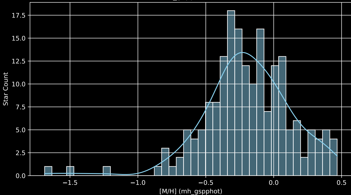
APOGEE DR17 Field: [K2_C8_140-55 [M/H] (mh_gspphot) (n= 188)
